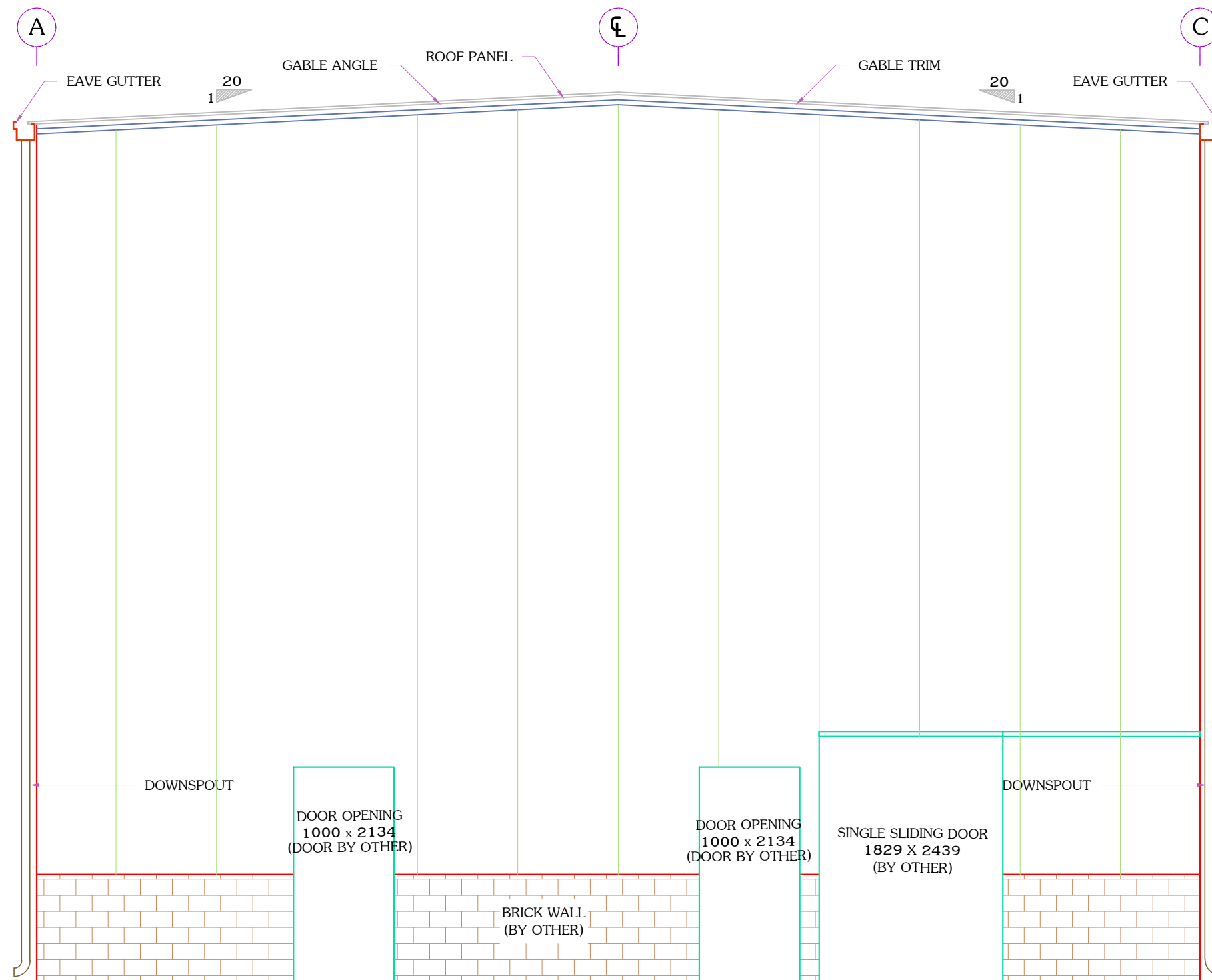
END WALL SHEETING @ GRID-1
